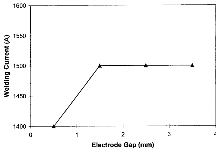
Fig. 8. Effect of electrode gap on the maximum welding current without sticking.
